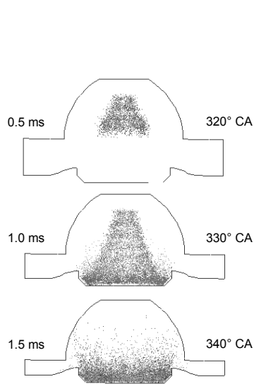
Fig. 9. Calculation of spray characteristics inside combustion chamber during compression stroke at 3333 RPM. Injection starts at 316^\circ CA and ends at 336^\circ CA.
