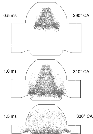
Fig. 10. Calculation of spray characteristics inside combustion chamber during compression stroke at 6666 RPM. Injection starts at 272^\circ CA and ends at 312^\circ CA.
